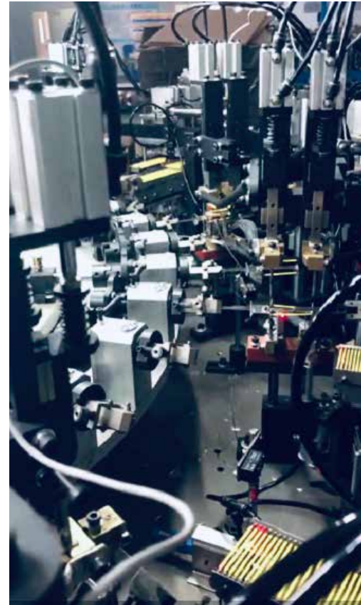
Spot Welding
